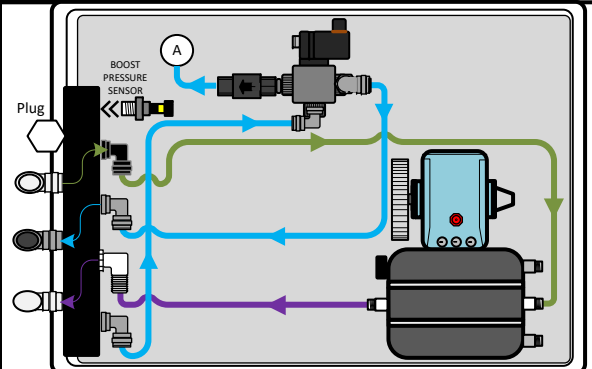
Detail View 2: Feed Pump Module Plumbing
