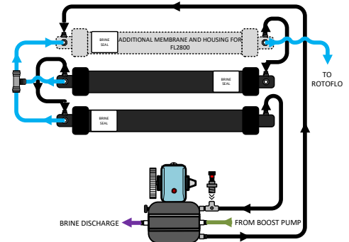
DETAIL VIEW 5: FL2800 Membrane Array Plumbing
