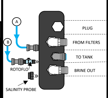
Detail View 1: Plumbing Manifold
