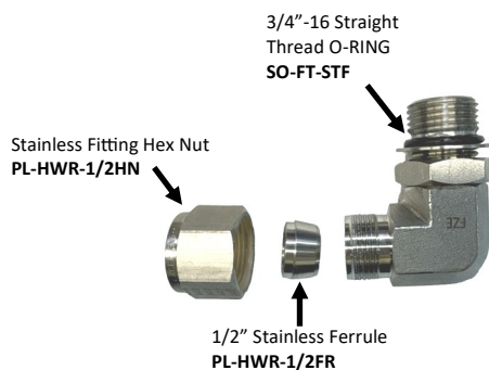
PL-MTS-3/8X1/2SL 3/8" NPT X 1/2" TUBE FITTING ST. SS316L
