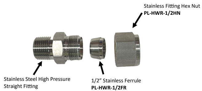
PL-MTE-3/4SX1/2SL 3/4"-16S X 1/2" TUBE 90DEG. SS316L
