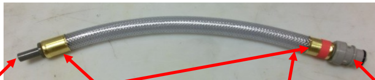
PL-HF-.75IDX1BR Brass ferrules for 1/2-inch hose
