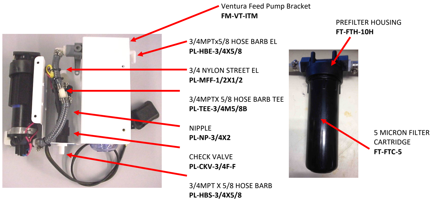
Pump Head Assembly W/Press. Switch PL-PMP-SFPH
