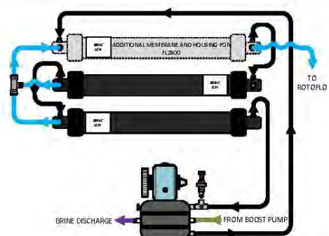
DETAIL VIEW 5: FL2800 Membrane Array Plumbing
