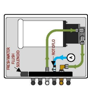
Detail View 2: Feed Pump Module Internals
